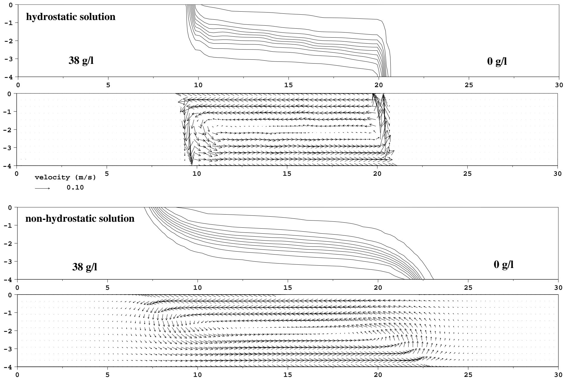
FIGURE 2: Lock exchange test-case. Comparison of hydrostatic and non-hydrostatic solutions
